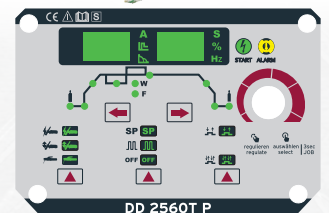
Operating panel DD 2560T P
