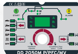
Operating panel DD 2050M P/PFC/MV
