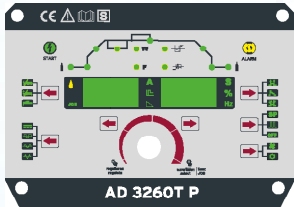
Operating panel AD 3260T P
