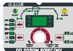
Operating panel DD 2050M P/PFC/MV Operating panel DD 2560T P
